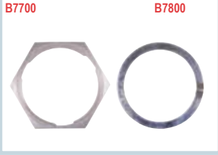
B7700 B7800 Order No. F-B7700 Order No. F-B7800 112263-90 112264 Fits all Deutsch Shell Size 24 Example: HD34-24-21PN Price .....$3.15 Price.....$1.20
