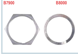
B7900 B8000 Order No. F-B7900 Order No. F-B8000 114020-90 114021 Fits all Deutsch Shell Size 18 Example: HD36-18-21PN Price .....$2.65 Price.....$1.15
